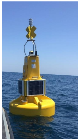
Figure 1. Buoy type SB138-P, diameter 1.75 m, focal height 2.9 m, yellow surface color with night signal flashlight
